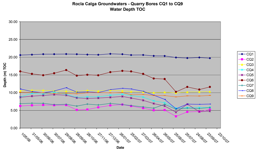
Figures 2 to 5: Groundwater Depth Charts.
